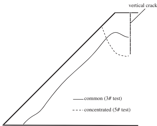
Fig. 5. Wetting fronts corresponding to different infiltration styles at a rainfall amount of 15 mm.
