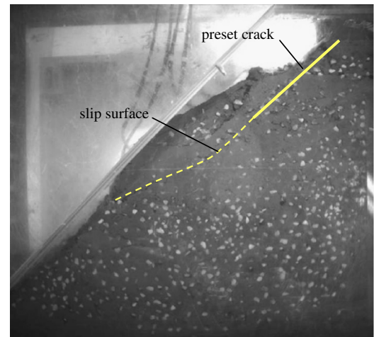
Fig. 12. Final failure of the slope with an oblique crack (4# test).
