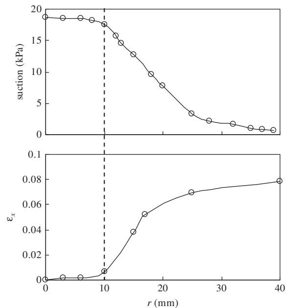
Fig. 3. Histories of horizontal strain and suction at #1 tensiometer's position in 2# tests. \epsilon_x , horizontal strain; r , rainfall amount.
