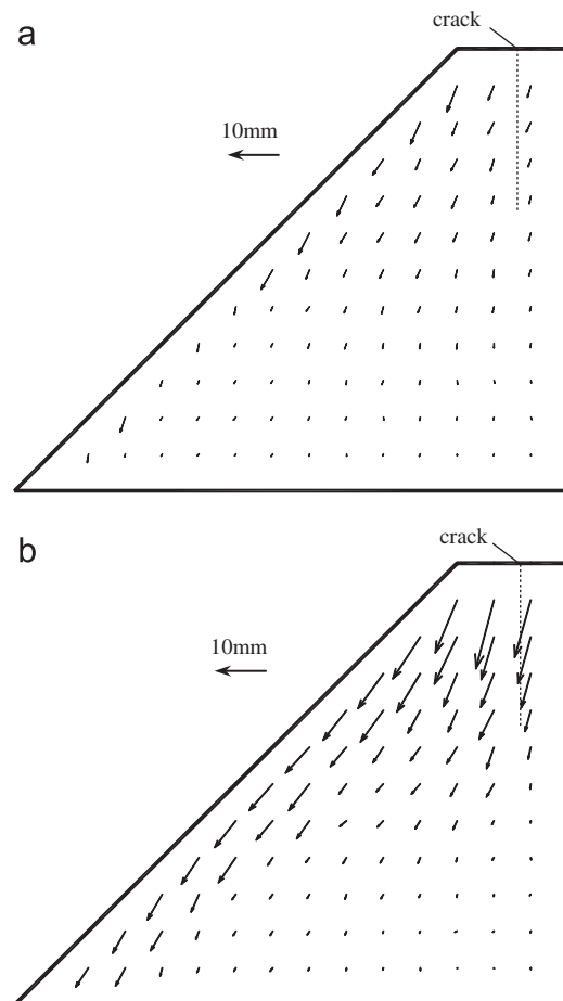
Fig. 6. Displacement vectors of the slope with a vertical crack at different rainfall amounts (3# test). (a) rainfall amount: 10 mm and (b) rainfall amount: 30 mm.
