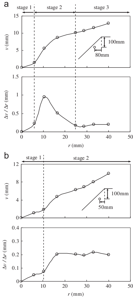
Fig. 7. Displacement histories of typical points of a slope with a vertical crack (3# test). v , vertical displacement; \Delta v/\Delta r , increase rate of vertical displacement; r , rainfall amount.
