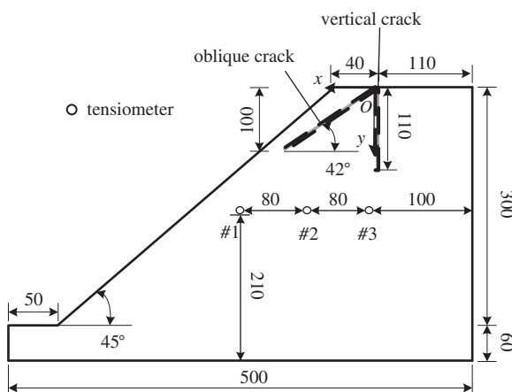
Fig. 1. Schematic view of the slope model (mm).
