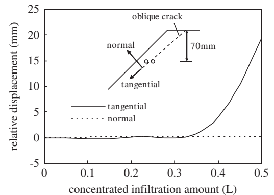
Fig. 13. Relative displacement history of a point couple along crack of the slope with an oblique crack (4# test). The horizontal distance between the measurement points and the crack was 5 mm.
