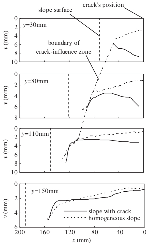
Fig. 8. Horizontal distributions of vertical displacement of homogeneous slope and of a slope with a vertical crack (3# test) at a rainfall amount of 20 mm. v , vertical displacement; x , horizontal coordinate; y , vertical coordinate.
