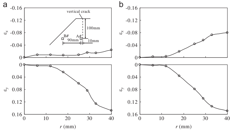
Fig. 9. Strain histories of typical points of the slope with a vertical crack (3# test). \varepsilon_x , horizontal strain; \varepsilon_y , vertical strain; r , rainfall amount. (a) element A# and (b) element B#.
