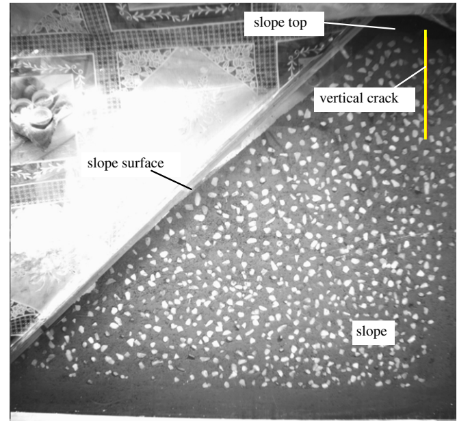
Fig. 2. Photograph of a typical slope model.
