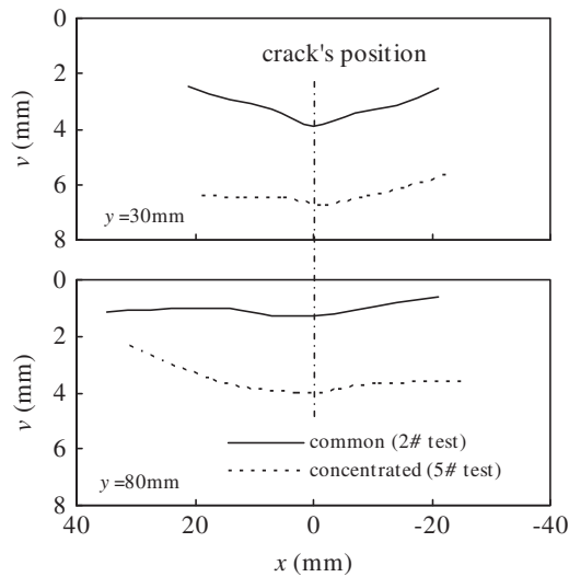
Fig. 10. Horizontal distributions of the vertical displacement of the slope with a vertical crack using different rainfall styles at an equivalent rainfall amount of 5 mm. v , vertical displacement; x , horizontal coordinate; y , vertical coordinate.
