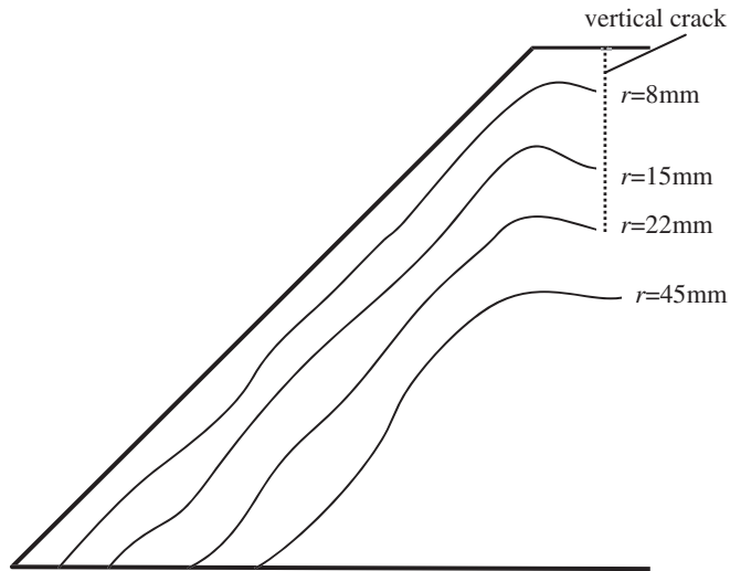
Fig. 4. Development of wetting fronts of the slope with a vertical crack (3# test). r , rainfall amount.
