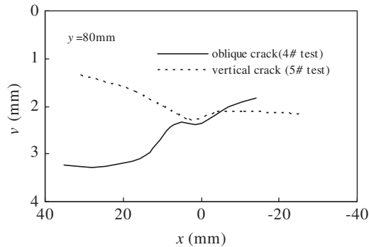
Fig. 11. Horizontal distribution of the vertical displacement of slopes with vertical and oblique cracks at a concentrated infiltration amount of 0.35 L. v , vertical displacement; x , horizontal coordinate; y , vertical coordinate.
