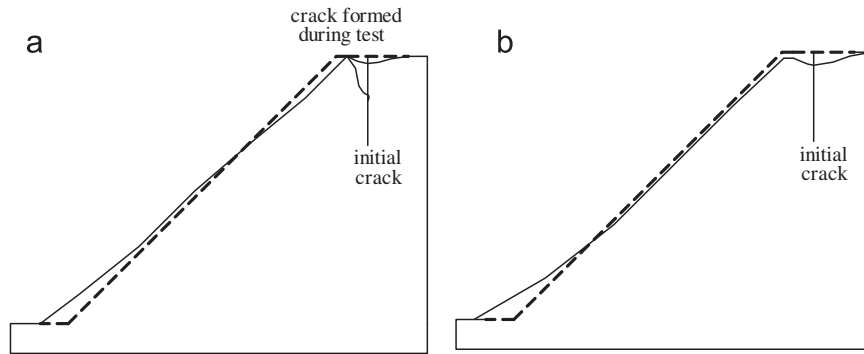
Fig. 14. Final failure of the slope with vertical cracks. (a) concentrated infiltration (5# test) and (b) common rainfall (2# test).
