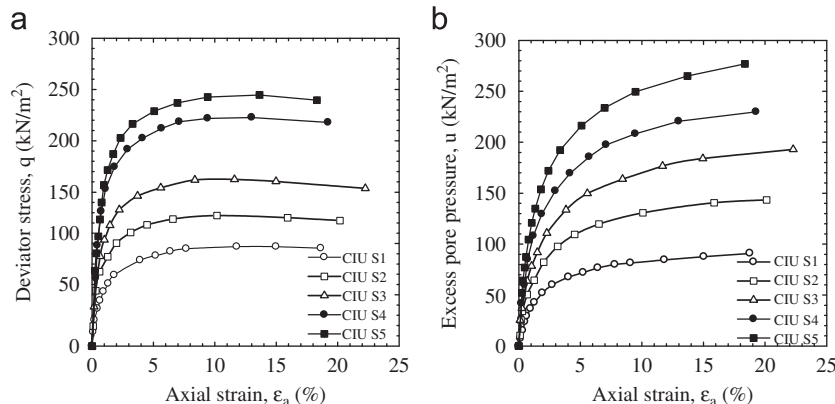
Fig. 7. Results of CIU triaxial tests on soft Bangkok clay. (a) Deviator stress versus axial strain and (b) Pore pressure versus axial strain.
