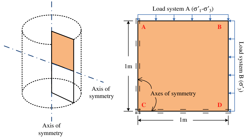
Fig. 13. Simplified geometries of triaxial test in finite element models.
