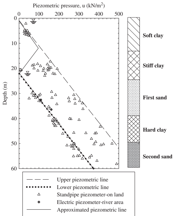
Fig. 2. Piezometric pressure in Bangkok subsoils.
